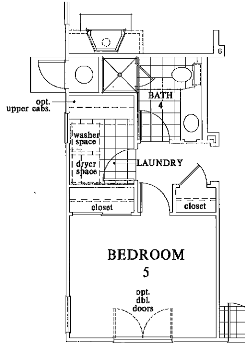
OPT. BDRM. 5 AT DEN WITH OPT. BATH 4 AT POWDER
